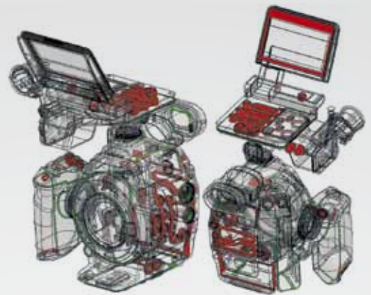
Dust-proof, splash-proof design ■ Sealed areas
